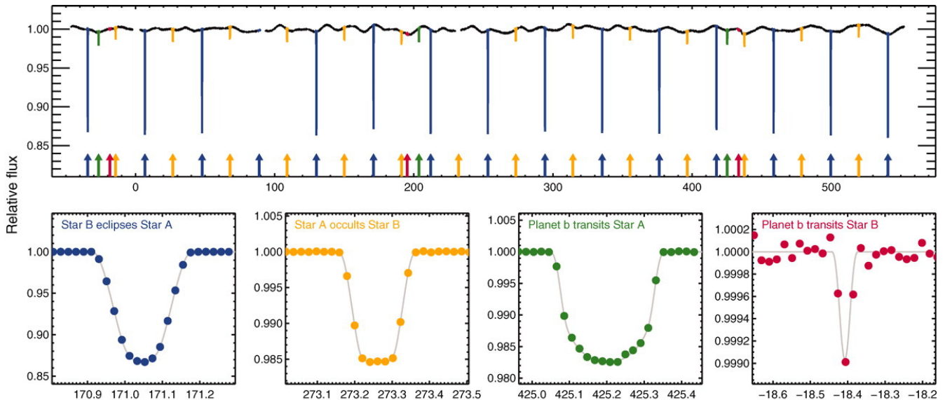
Figure 1: The light curve of Kepler 16 showing the stellar eclipses (blue and yellow) as well as the transits of the planet across the stellar disks (green and red). Note that there is variability outside the eclipses, presumably due to the migration of starspots across the primary star's surface.
